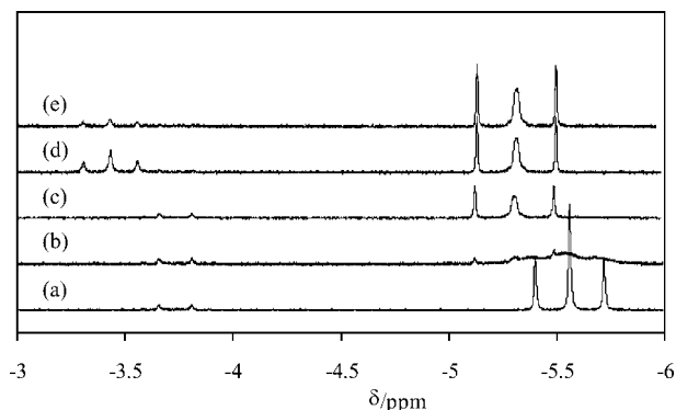
Figure 5. ^1\text{H} NMR (300 MHz) spectroscopic monitoring of the reaction between [\text{Cp}^*\text{Mo}(\text{dppe})\text{H}_3] and TFA in [\text{D}_8]\text{thf} (290 K): (a) before the TFA addition; (b) TFA/Mo = 0.5, 8 min; (c) further addition of 1 equiv. to sample (b): TFA/Mo = 1.5, 30 min; (d) TFA/Mo = 10, immediately after the addition; (e) after 13 min from spectrum (d). The doublet resonance at \delta = -3.73 ppm belongs to the [\text{Cp}^*\text{Mo}(\kappa^1\text{-dppe})\text{H}_3] contaminant. [14]
