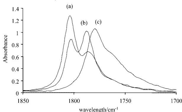
Figure 8. IR spectra of trifluoroacetic acid solutions ( 0.027\text{ M} , pathlength 0.04\text{ mm} ) in various solvents at 290\text{ K} : (a) \text{CH}_2\text{Cl}_2 ; (b) toluene; (c) THF.
