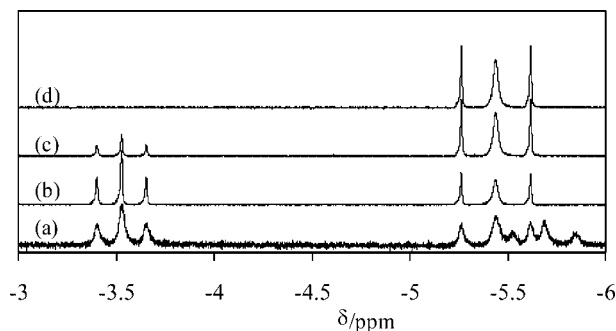
Figure 7. ^1\text{H} NMR-spectroscopic study of the [\text{Cp}^*\text{Mo}(\text{dppe})\text{H}_3]^+ –TFA reaction in [\text{D}_3]\text{MeCN} at room temperature: (a) 0.5 equiv. TFA, recorded immediately; (b) 1 equiv. TFA, recorded immediately; (c) after 9 min from spectrum (b); (d) 40 min after spectrum (b).
