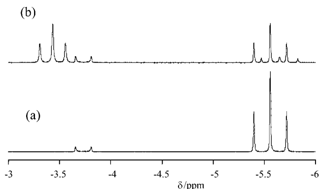
Figure 6. ^1\text{H} NMR-spectroscopic study of a [\text{Cp}^*\text{Mo}(\text{dppe})\text{H}_3]/\text{HBF}_4 mixture in [\text{D}_8]\text{thf} : (a) starting compound; (b) 21 min after the addition of 0.5 equiv. \text{HBF}_4 . The doublet resonance at \delta = -3.73 ppm belongs to the [\text{Cp}^*\text{Mo}(\kappa^1\text{-dppe})\text{H}_3] contaminant. [14]
