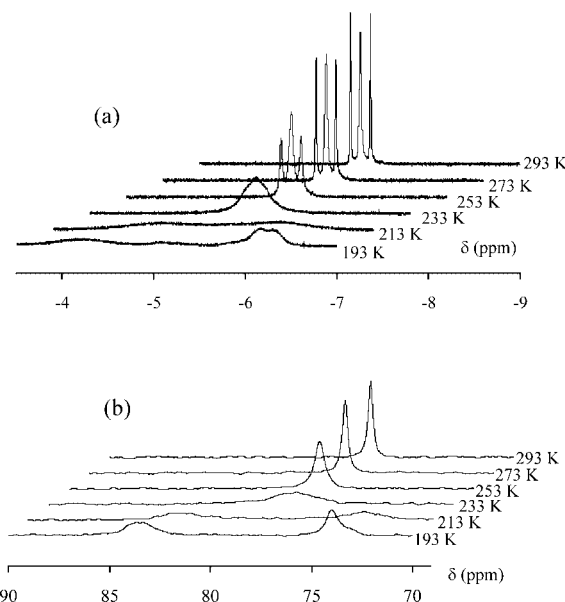
Figure 1. Variable-temperature spectra for compound [\text{Cp}^*\text{Mo}(\text{dppe})\text{H}_2(\text{O}_2\text{CCF}_3)] in \text{C}_6\text{D}_5\text{CD}_3 : (a) ^1\text{H} NMR (500 MHz); (b) ^{31}\text{P}\{^1\text{H}\} NMR (202 MHz).
