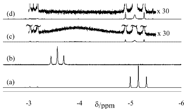
Figure 3. ^1\text{H} NMR (300 MHz) spectroscopic monitoring of the reaction between [\text{Cp}^*\text{Mo}(\text{dppe})\text{H}_3] and TFA in \text{C}_6\text{D}_6 (290 K): (a) starting material before the TFA addition; (b) immediately after the TFA addition (10 equiv.); (c) immediately after the TFA addition (1 equiv.); (d) after 3.5 h from spectrum (c).
