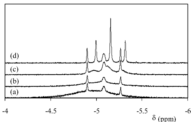
Figure 4. ^1\text{H} NMR (300 MHz) spectroscopic monitoring of the reaction between [\text{Cp}^*\text{Mo}(\text{dppe})\text{H}_3] and TFA (1:0.5 ratio) in \text{C}_6\text{D}_6 (290 K): (a) recorded immediately; (b) after 7 min; (c) 28 min; (d) 155 min.
